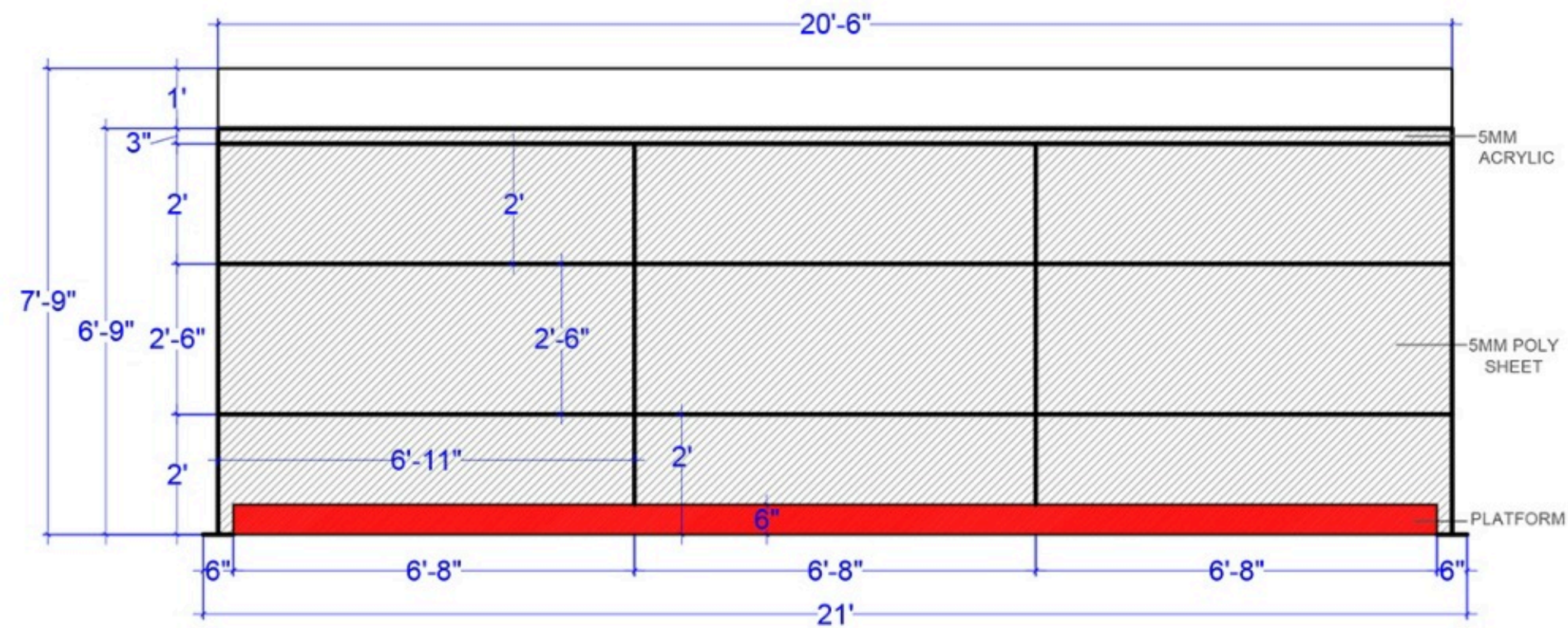
FRONT ELEVATION
